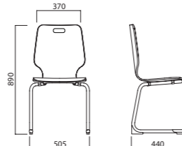
JENNY REVERSE CANTILVER ALU
